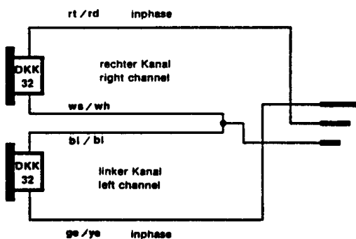
Wiring diagram old K 141 Versions
