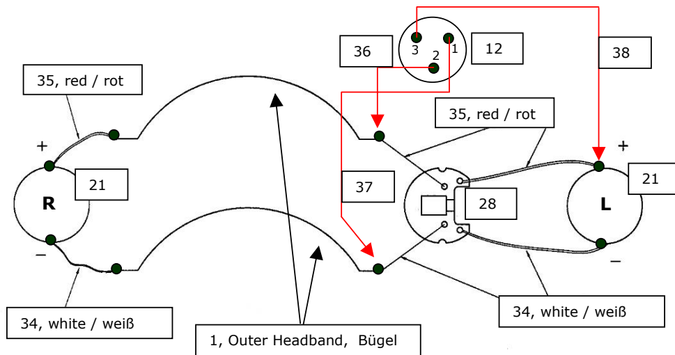
Wiring diagram old K 141 Versions
