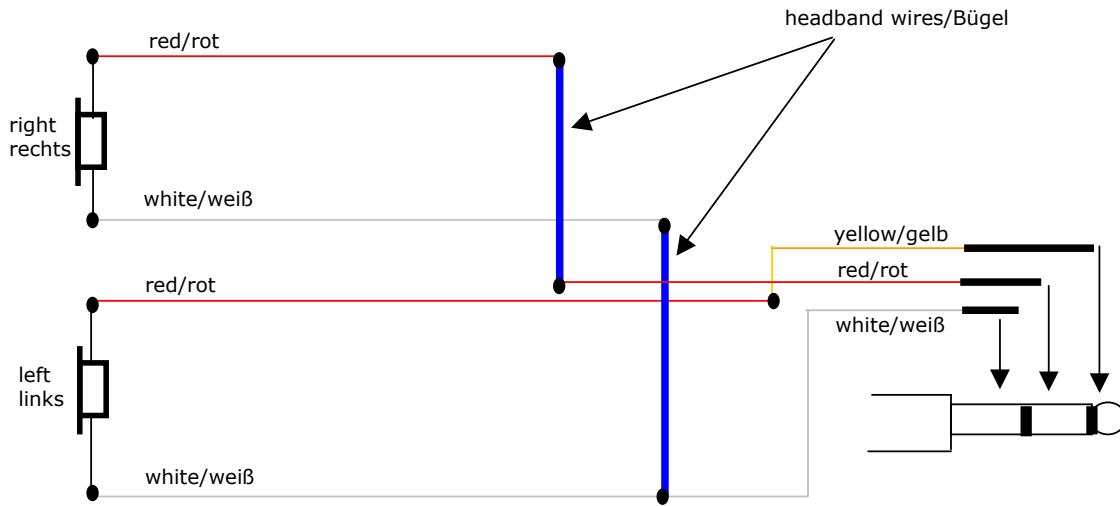
Wiring diagram K 141 Studio / K 141 Studio II
